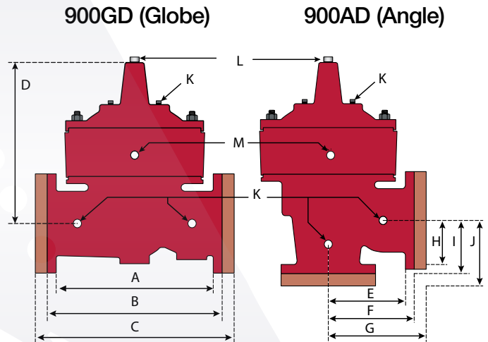
Model 900GD: Globe Pattern Dual Chamber Basic Valve
