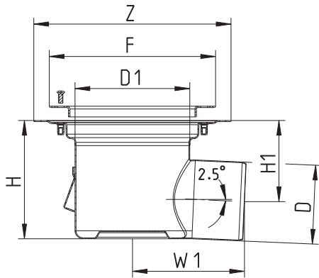
Side Outlet
