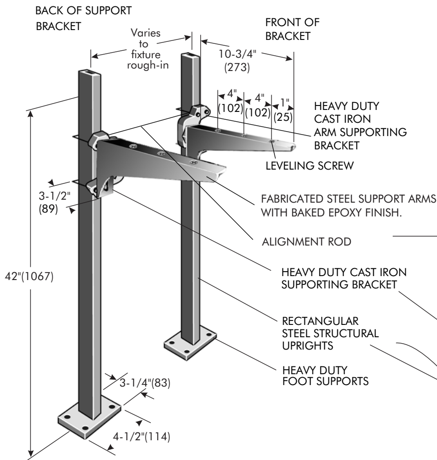
CA-402-D (DETAIL) The CA-402-D is furnished with opposed arms mounted on uprights with back to back heavy duty cast iron support brackets
