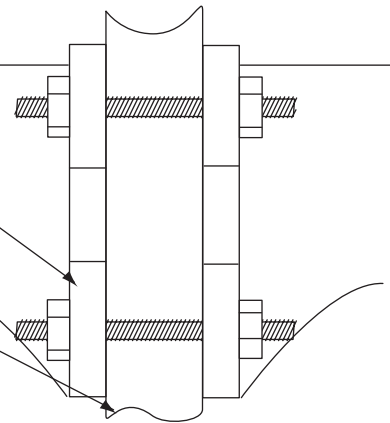
CA-402-D (DETAIL) The CA-402-D is furnished with opposed arms mounted on uprights with back to back heavy duty cast iron support brackets
