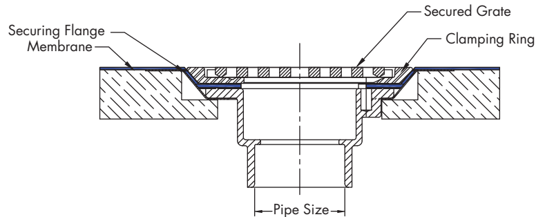
Typical Installation
