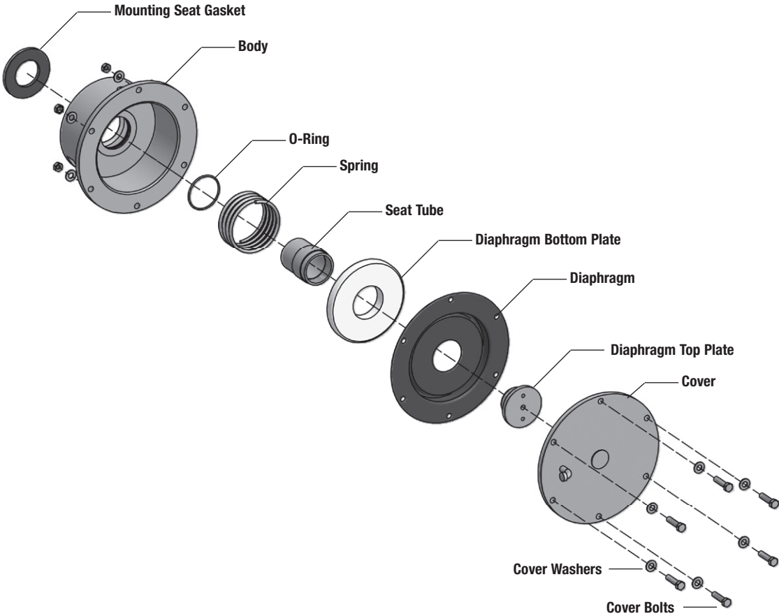
4" – 10" 4000/5000 Relief Valve (Note: Mounting Bolts not shown)
