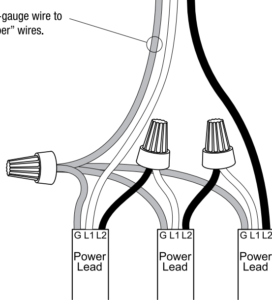
Schematic showing how to connect three heating mats or cables to the LoudMouth for monitoring during installation.
