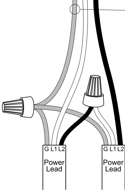
Schematic showing how to connect two heating mats or cables to the LoudMouth for monitoring during installation.
